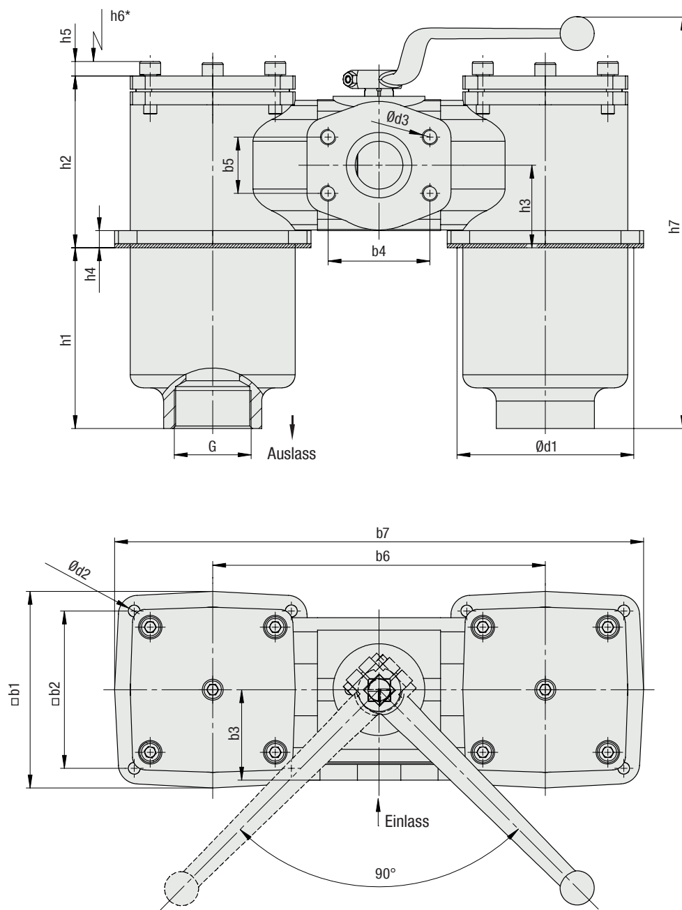
RFS-D-090/160
