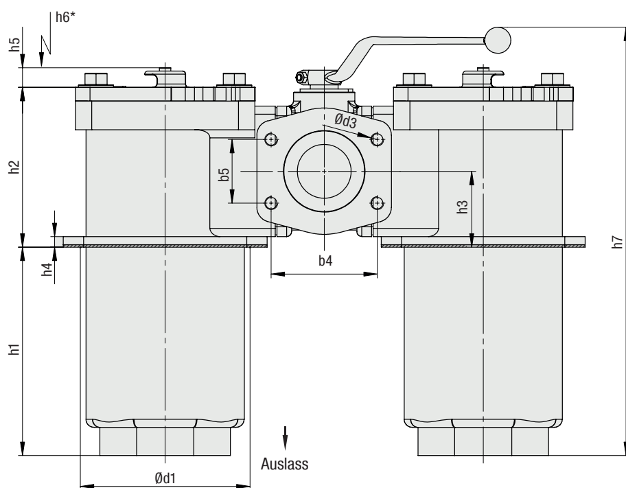
RFS-D-250/300
