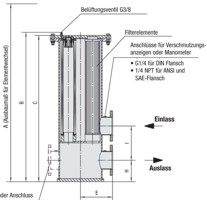
SRFL-S-3600
