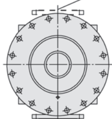
Ablassventil G1/2
