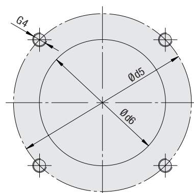
Mounting Detail
